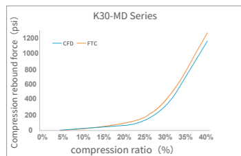
FTC- Force to Compress CFD- Compression Deflection
